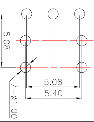
PCB layout (Pattern Side)
